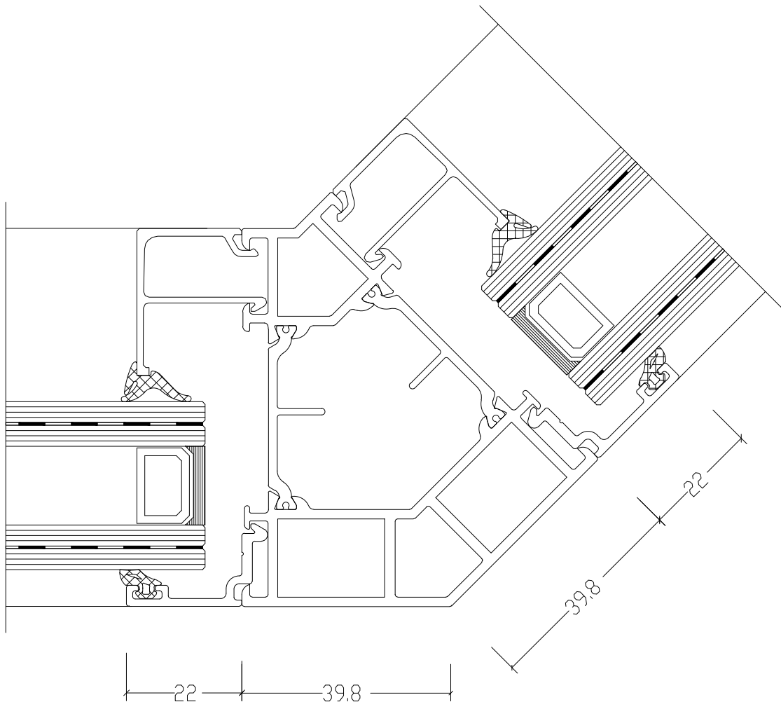
45 graden hoekoplossing
