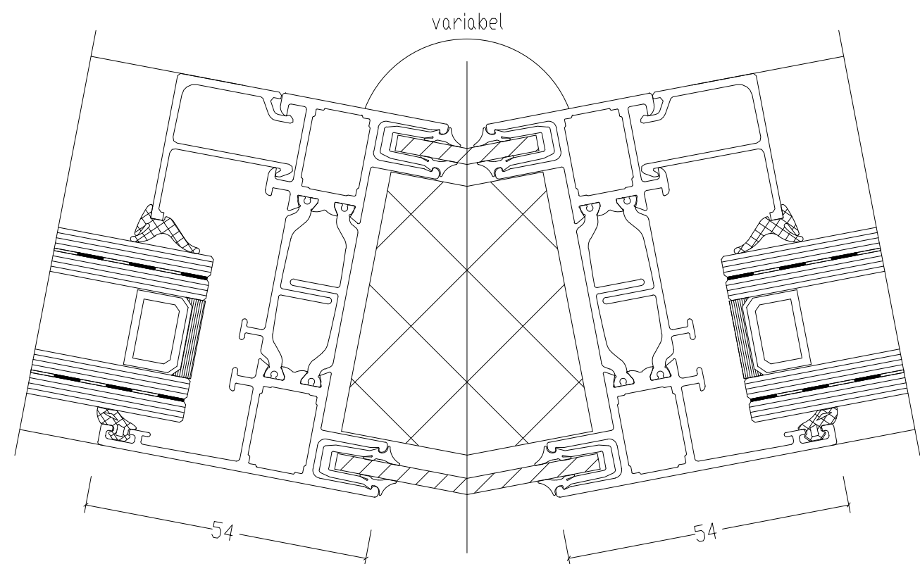
Variabele hoekoplossing
