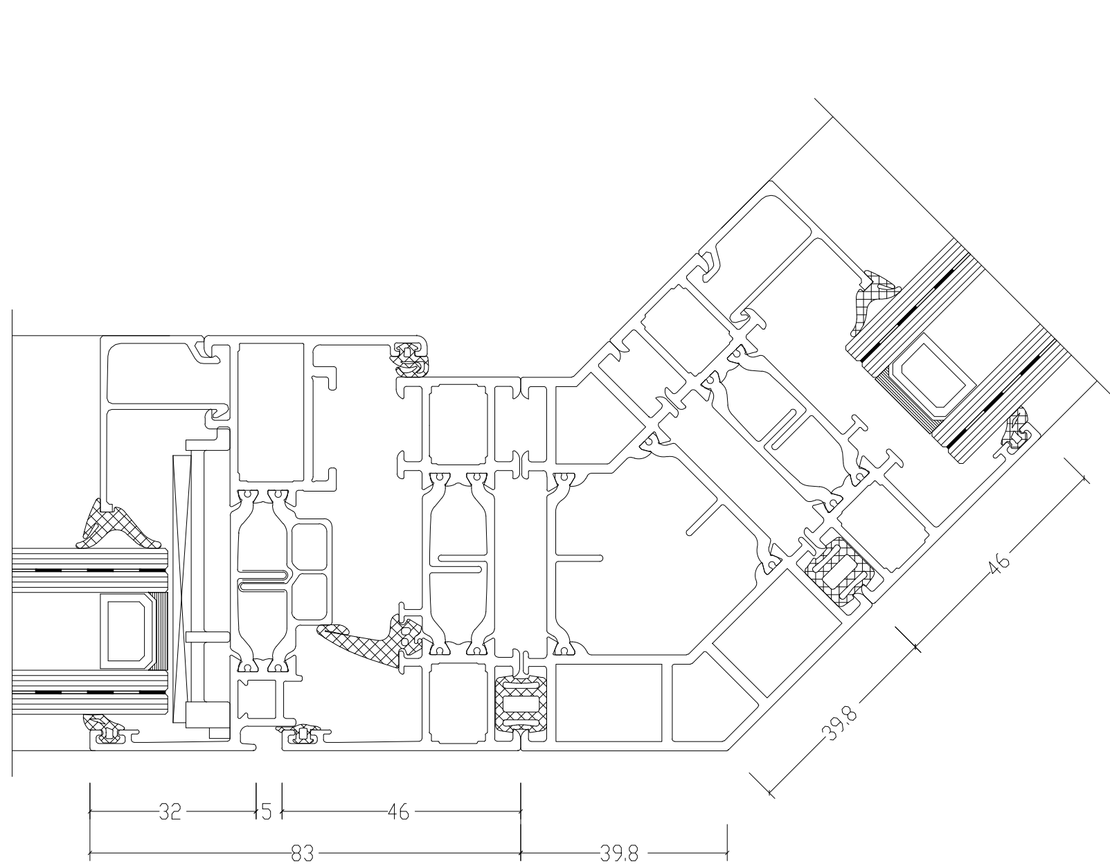
45 graden koppeling
