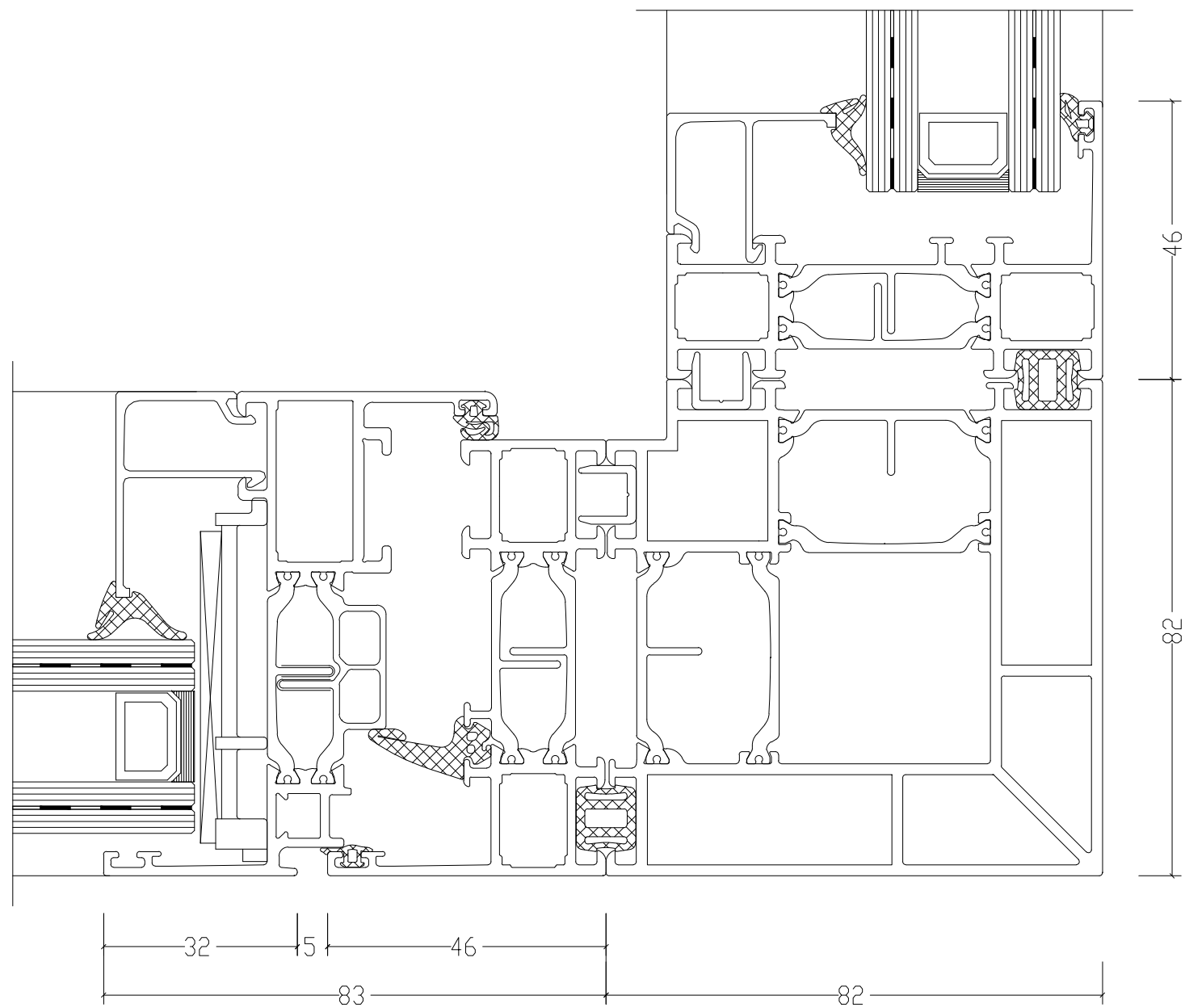
90 graden koppeling
