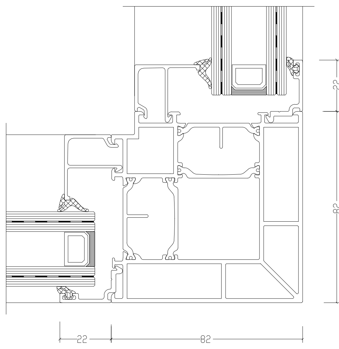
90 graden hoekoplossing
