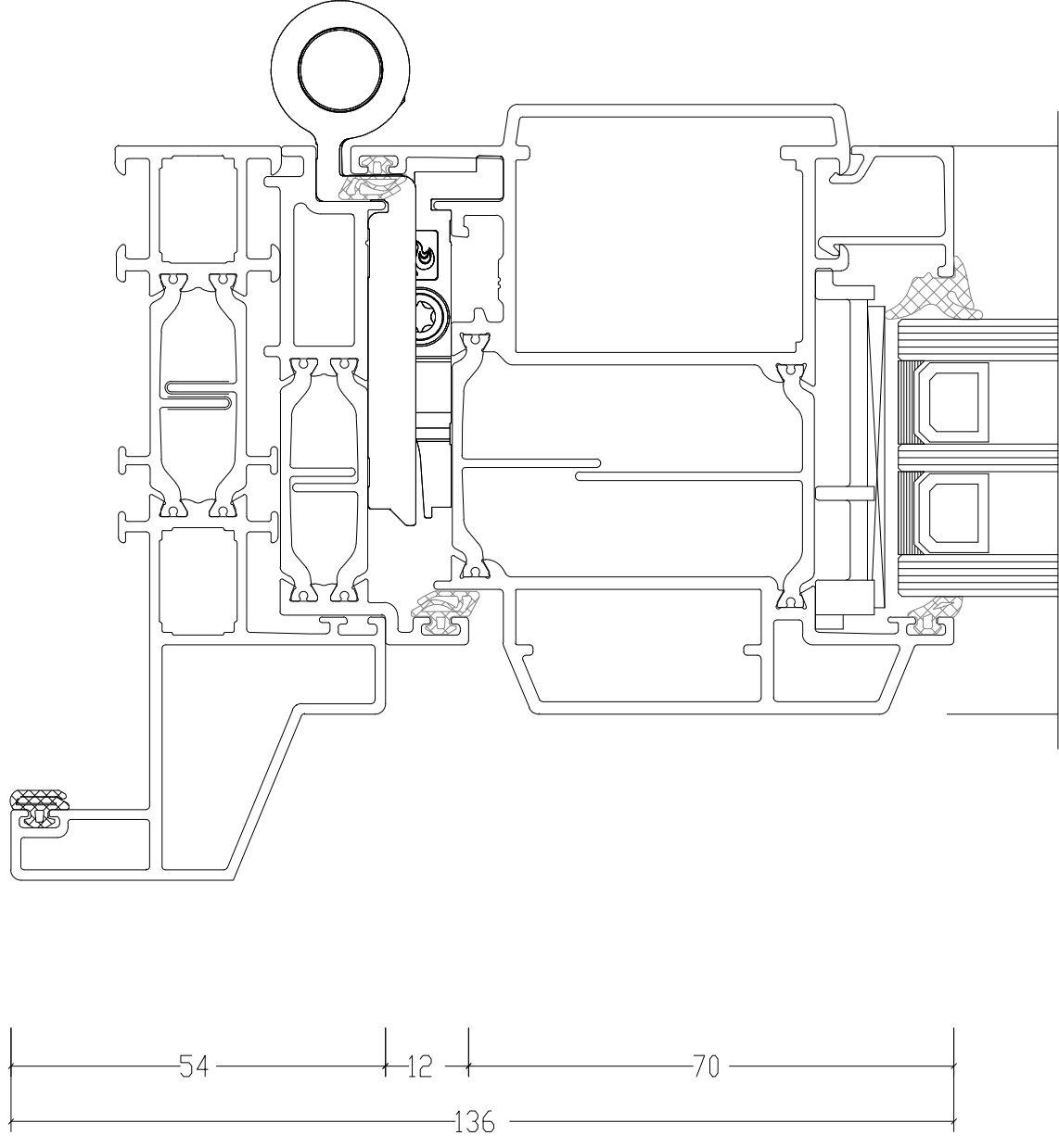
TRIPLE GLAS
