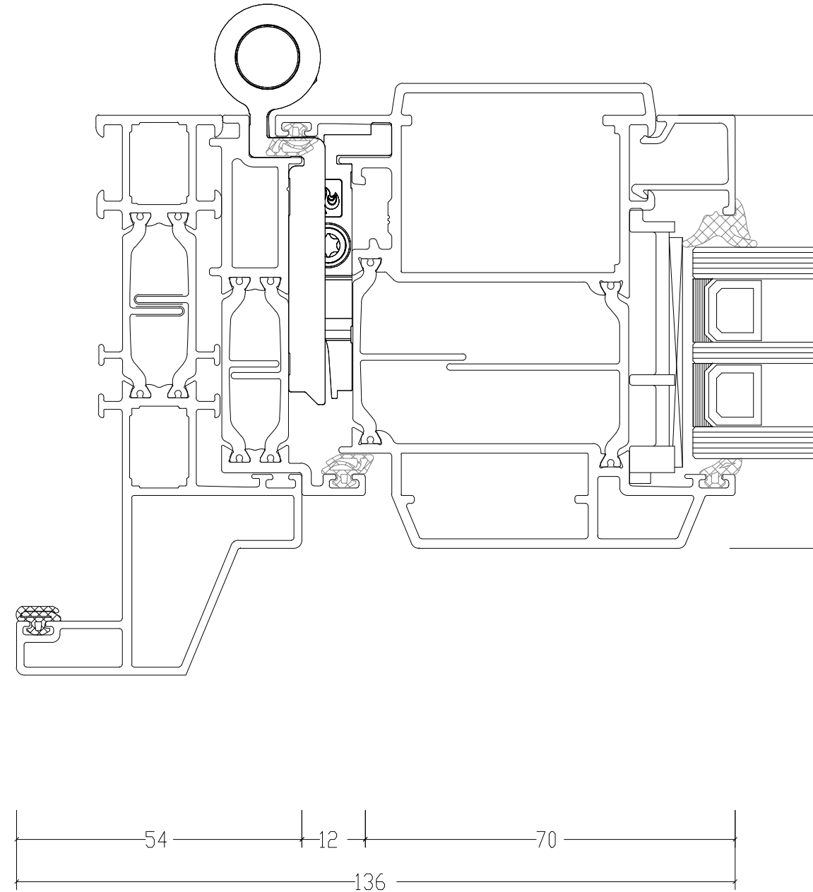
TRIPLE GLAS
