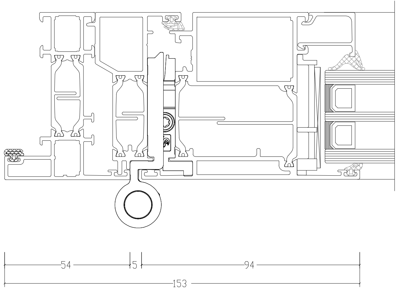
TRIPLE GLAS
