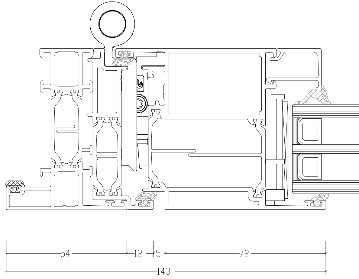
TRIPLE GLAS
